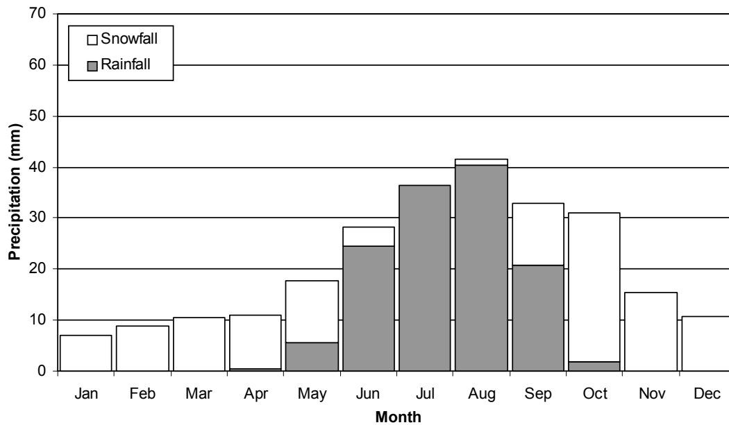
(a) Mean Monthly Recorded Precipitation at Contwoyto Lake Period of Record 1959 to 1981
