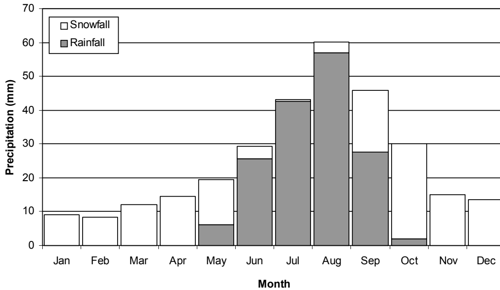
(b) Mean Monthly Recorded Precipitation at Lupin Period of Record 1982 to 2001
