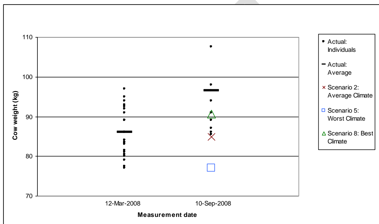
Figure 12. Comparison of predicted and actual body weights. Actual weights were recorded for adult (age 3+) cows from the Bathurst herd in 2008 on 2 different dates. Predicted weights are displayed for the 3 scenarios representing current development (i.e. scenarios 2, 5, and 8) for September 10 th .
