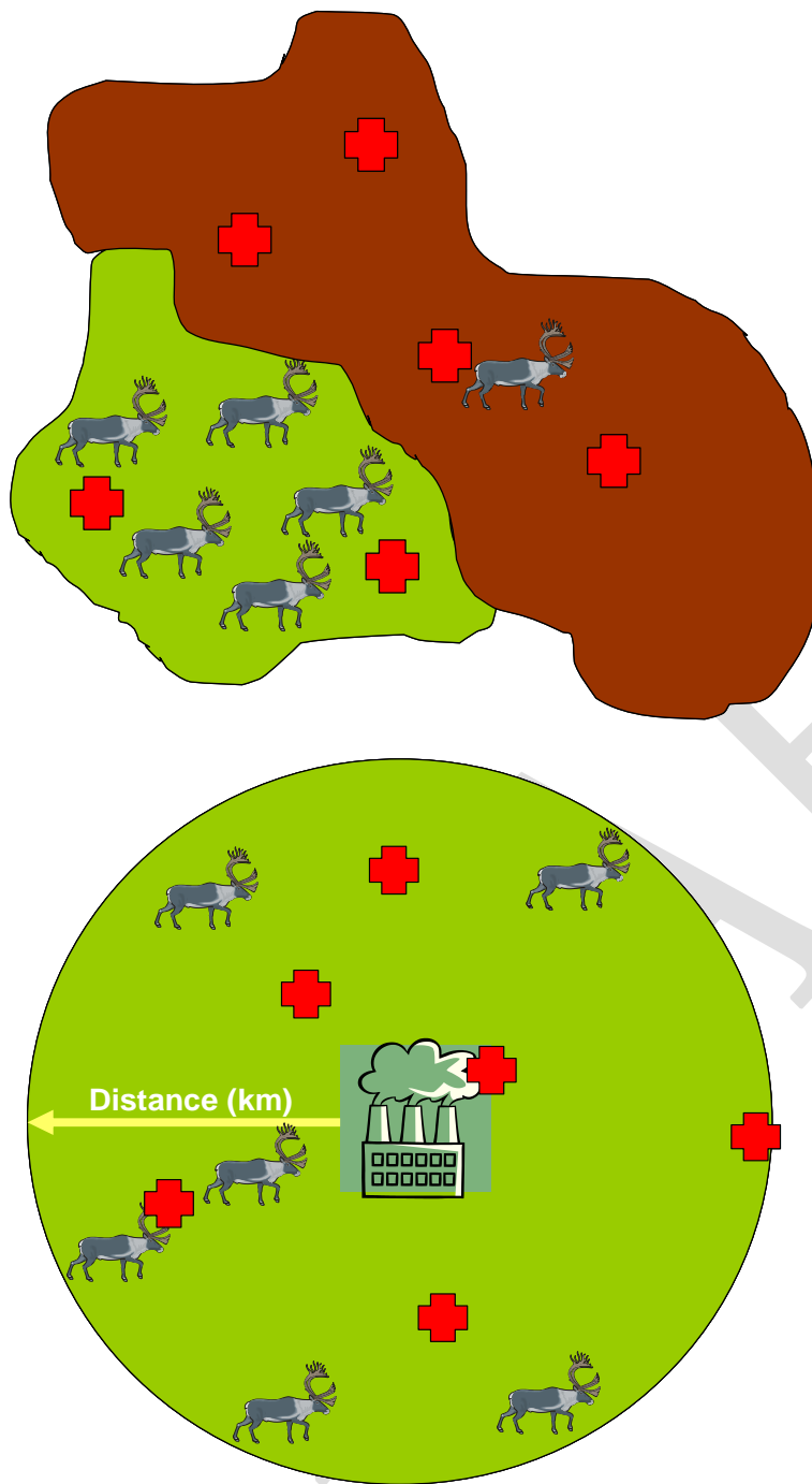
Figure 2. Distribution of caribou quantified using a hypothetical resource selection function. In the top panel, a greater proportion of caribou locations in the green habitat would reveal habitat selection and a positive weighting coefficient. Distribution of caribou quantified using a hypothetical resource selection function. In the top panel, a greater proportion of caribou locations in the green habitat would reveal habitat selection and a positive weighting coefficient. In the bottom panel, caribou are distributed farther from the factory relative to the random locations (red cross) suggesting avoidance of that feature.
