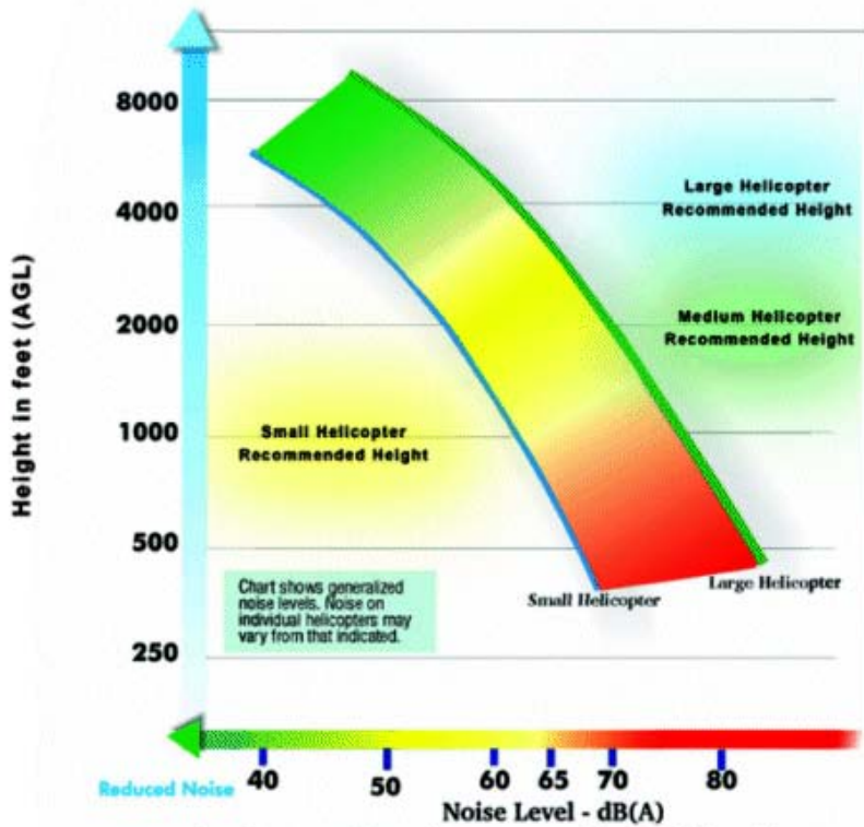
Variation of Noise Levels with Flyover Height
