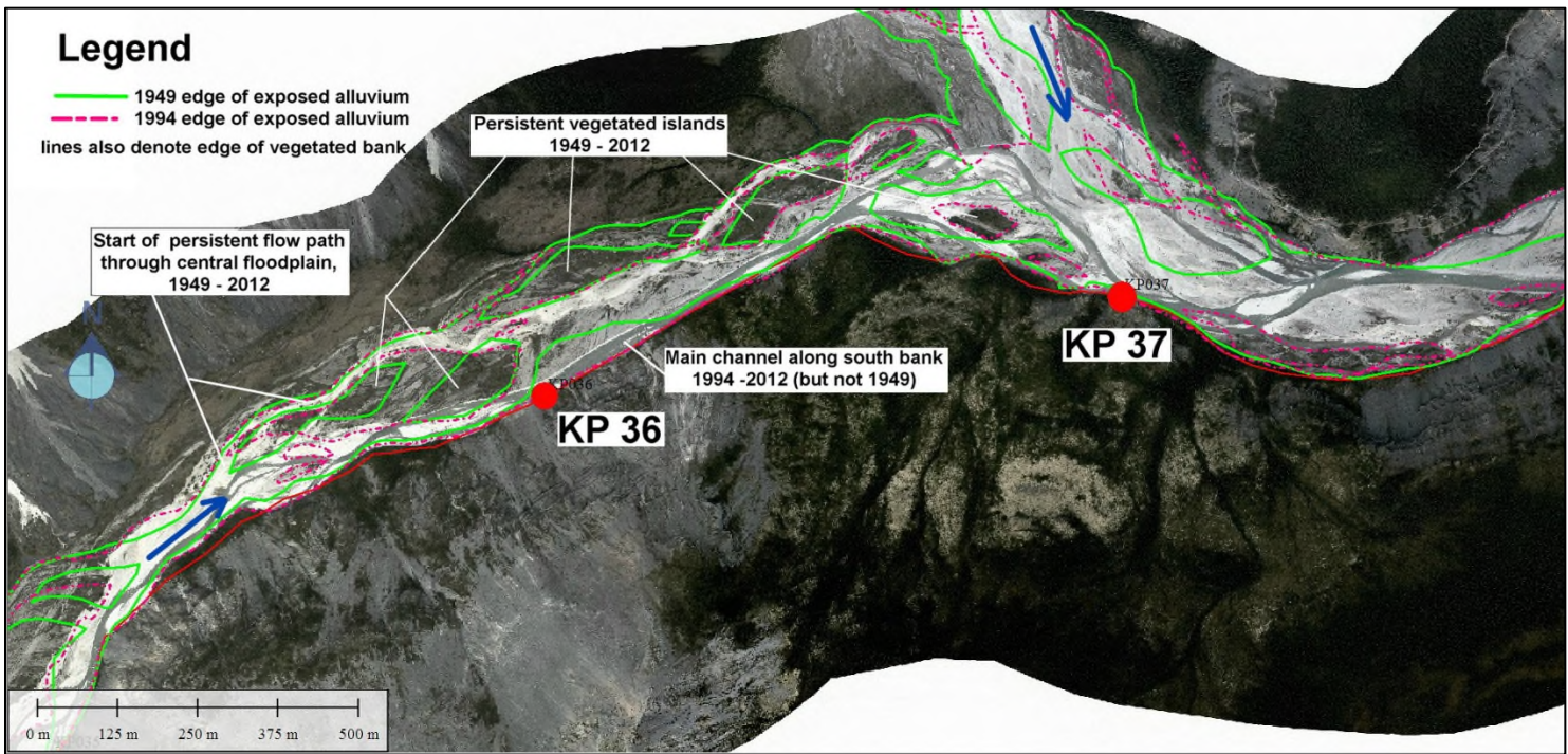
Channel movement: 1949 and 1994 bank edge shown on 2012 orthophoto
