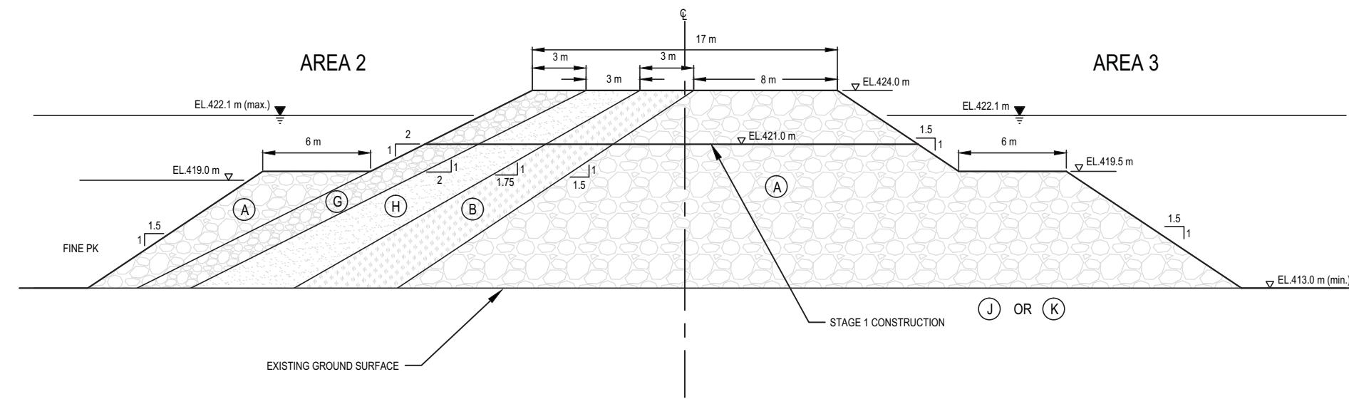
TYPICAL SECTION - DYKE L (INTERNAL FILTER DYKE)
