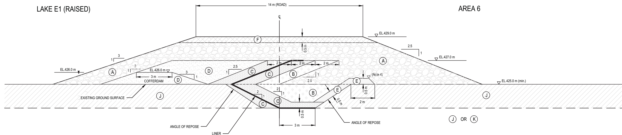
TYPICAL SECTION - DYKE G (DIVERSION DYKE)
