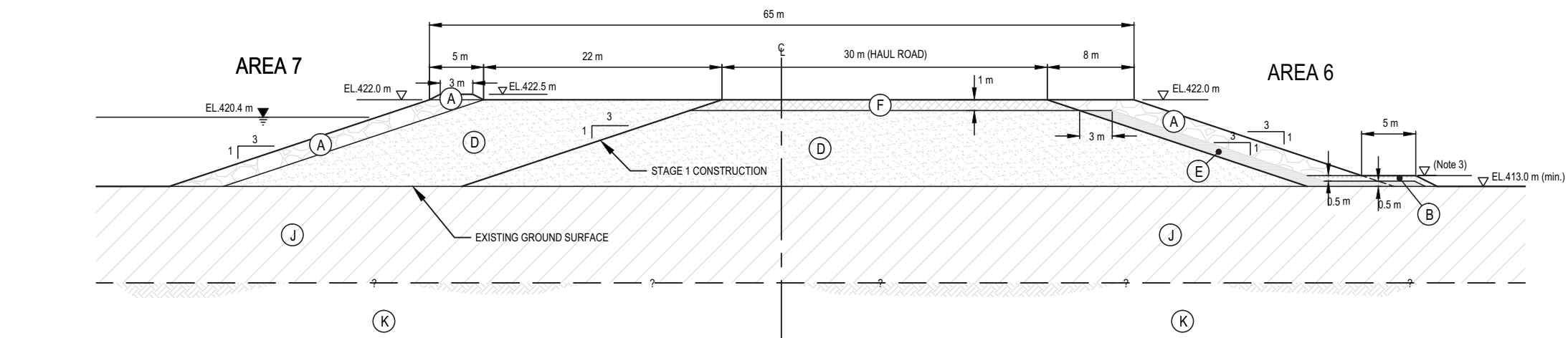
TYPICAL SECTION - DYKE K (INTERNAL WATER RETENTION DYKE)
