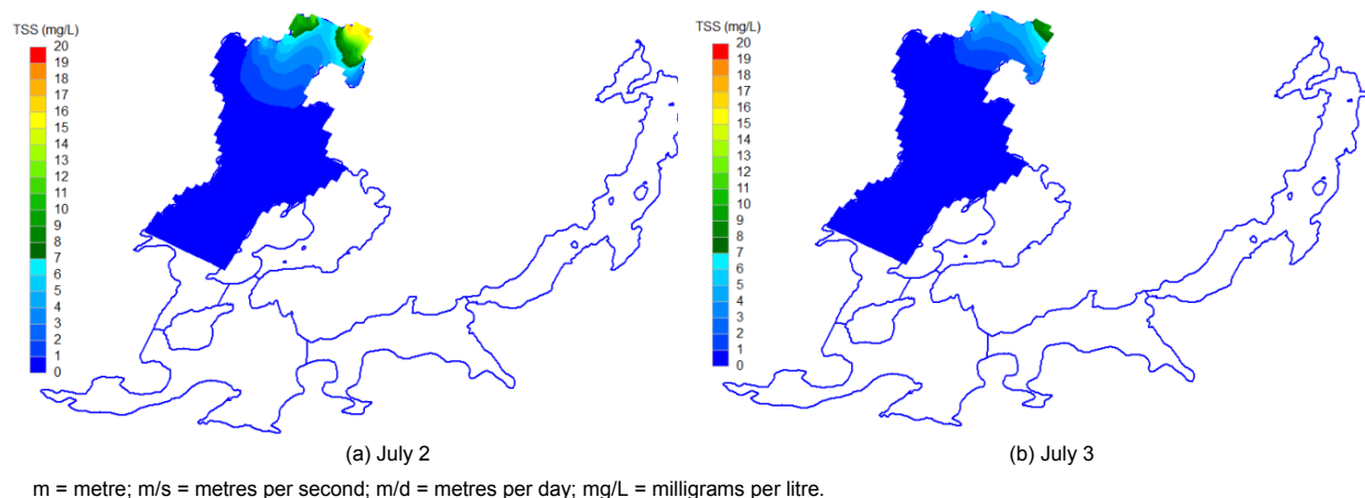
Figure 7 Total Suspended Solids Concentration in the Surface Layer of Area 2 and Areas 3 and 5 at an Elevation of 420.7 m after a Storm Event in the Open-water Season with a Wind Speed of 10 m/s from the Southwest and a Sediment Settling Velocity of 0.01 m/d
